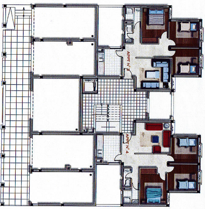
PLAN NIV +2.20
