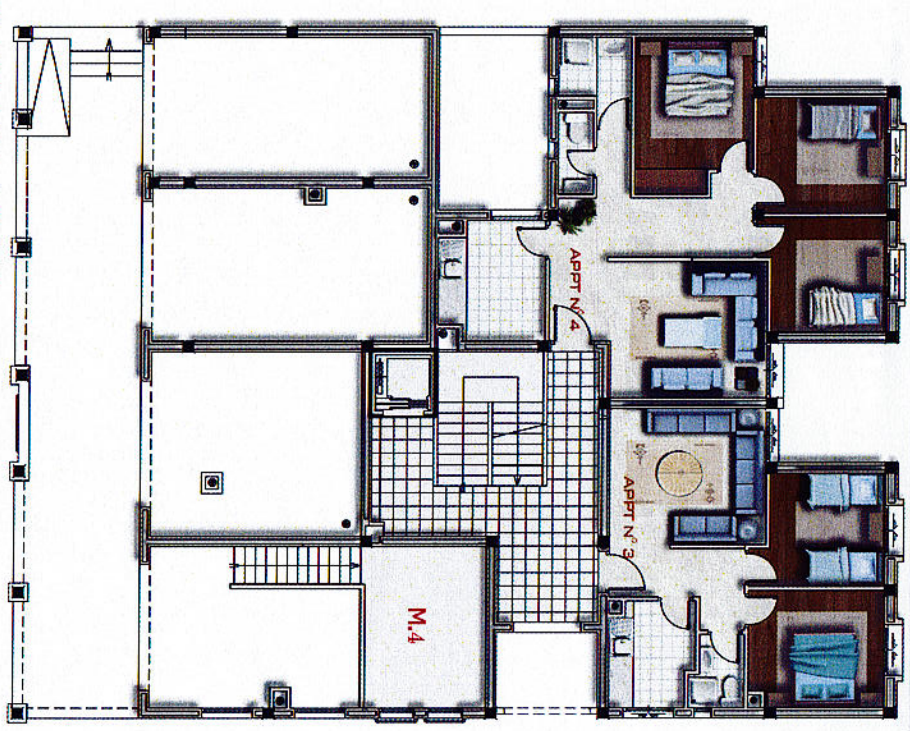
PLAN NIV +2.20
