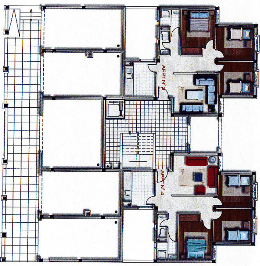
PLAN NIV +2.20
