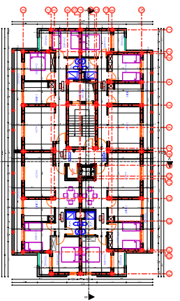
PLAN 4 EME ETAGE
