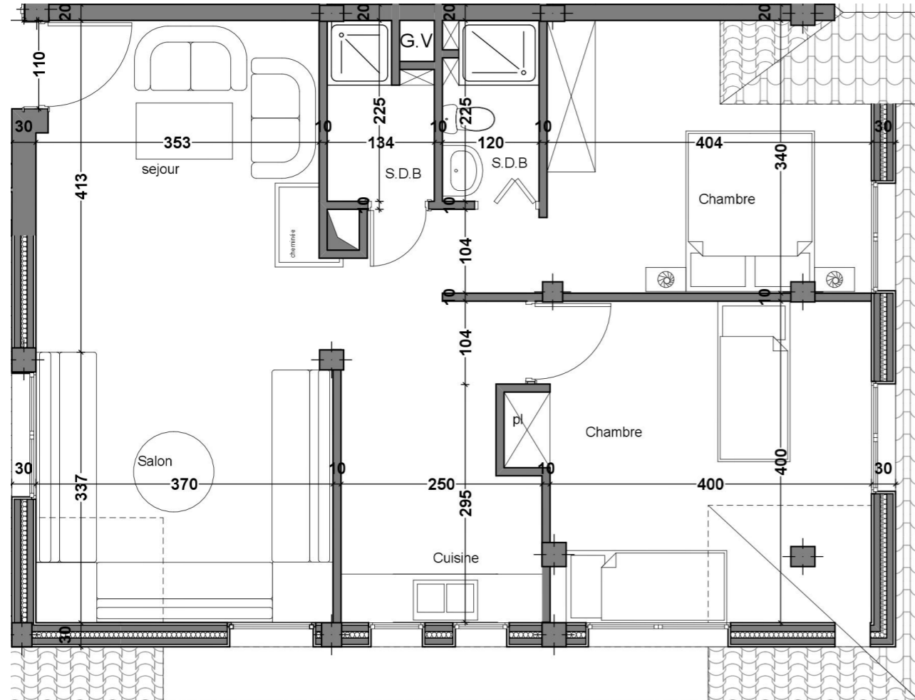
Apt 12
