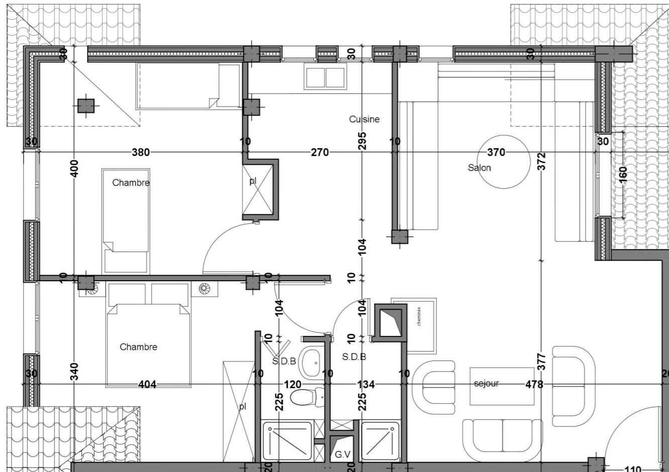
Plan Comble
