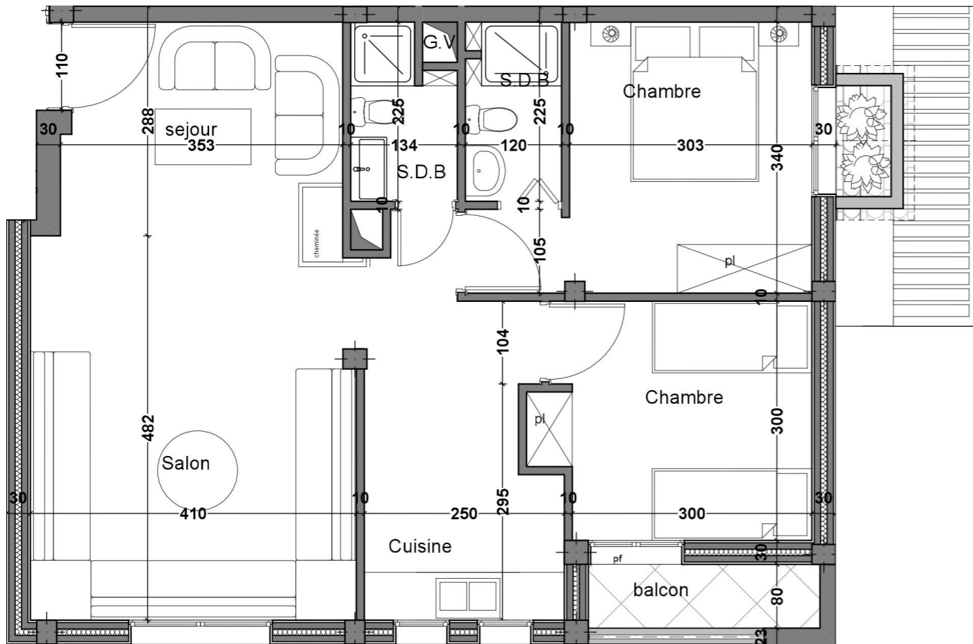
Apt 8
