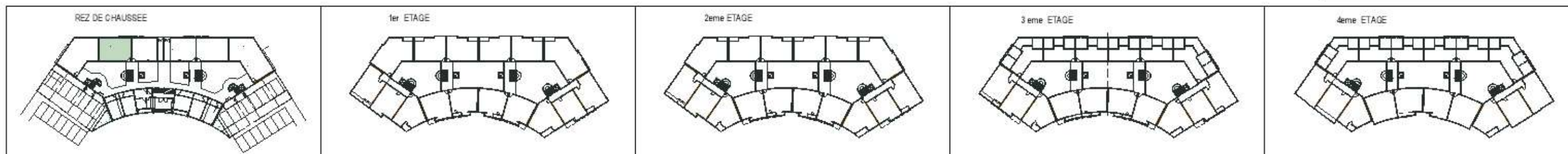
PLAN APPARTEMENT TYPE T 02 SURFACE = 63.00 m 2
