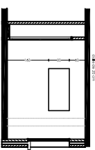
detail niche 2
